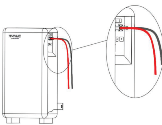
Fig.6-4 Power Cable Connection Diagram
