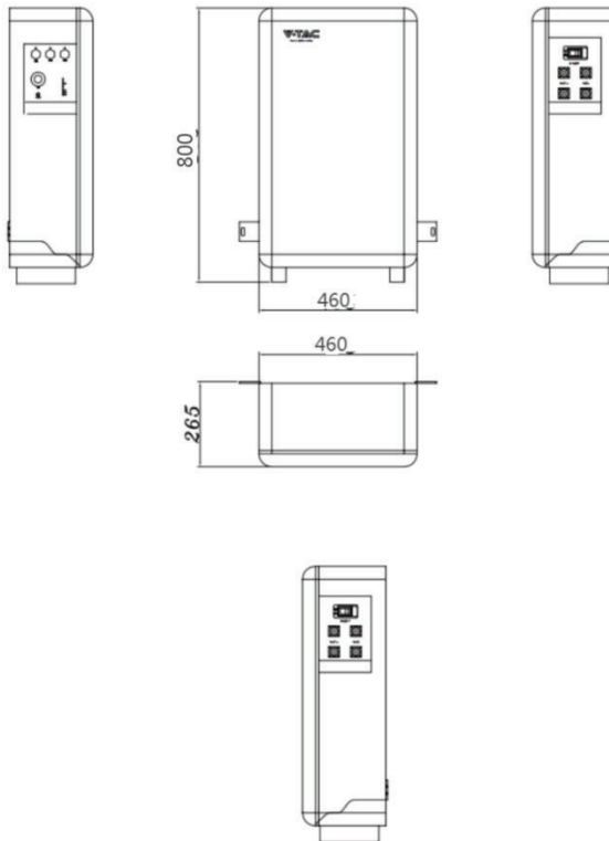
Fig. 5-1 Product Dimensions
